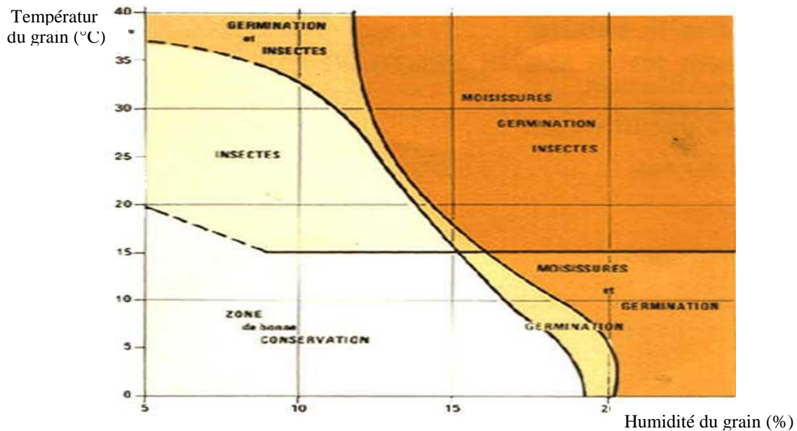
Figure I.6: Zone de stockage [3].
